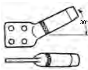
30° Palm bent on edge
