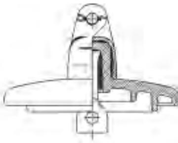
Tongue & Clevis (T & C)
