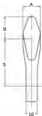
Fig. 2 Ball Hook Long Shank
